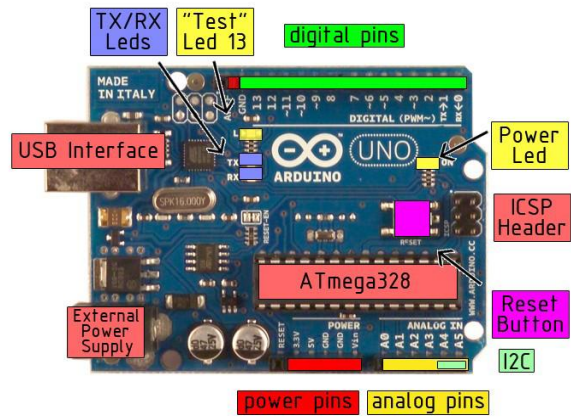
Fig.6 Arduino UNO board. How to use Arduino?
