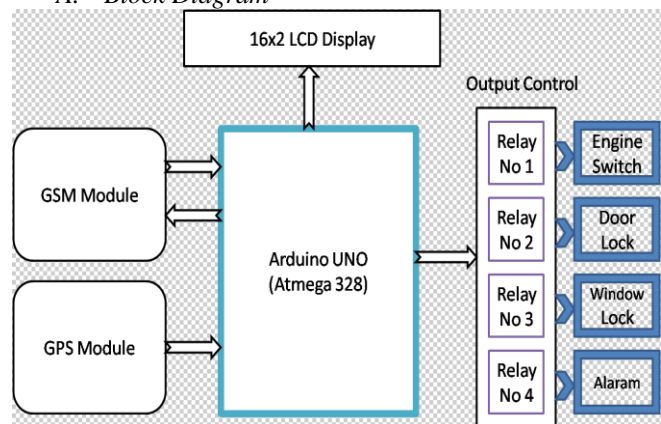
Fig.1 Block Diagram of Vehicle Tracking System.
