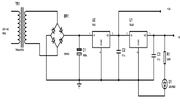
Fig.2 Power Supply Section
