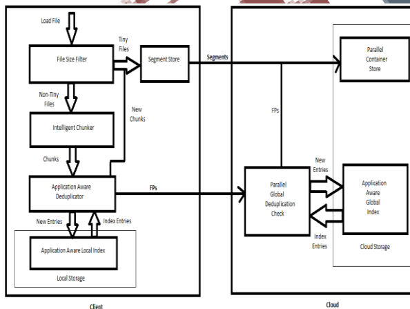
Fig 1. Architecture Overview of ALG-Dedupe Design
