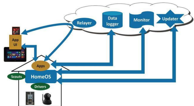
Fig. 1 LoT Architecture
