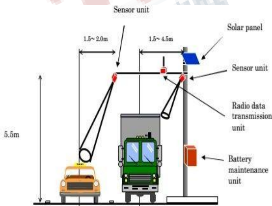
Fig. 1 Structure of sensor on street light
