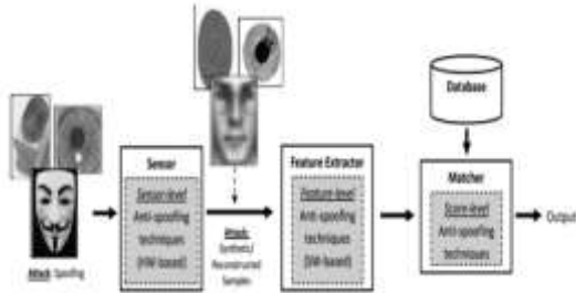
Fig.3: Anti-Spoofing Techniques
