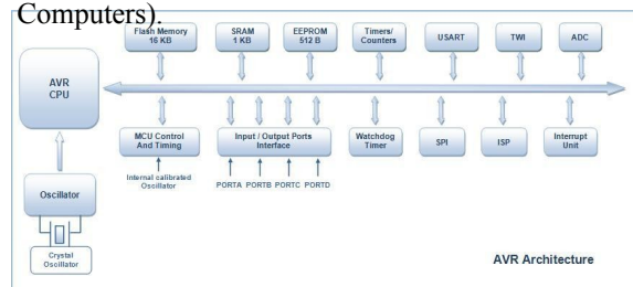
Figure 1: Architectural Diagram Of At Mega 16
