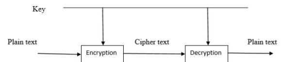
Figure 1: Symmetry Cryptography
