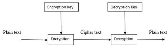
Figure 2: Asymmetric Cryptographic
