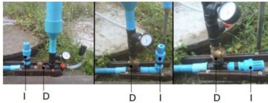
Figure 5. Different valve arrangement in the construction of a hydraulic ram (from left to right: I , IIv , IIh; eith I impulse valve; D delivery valve)
