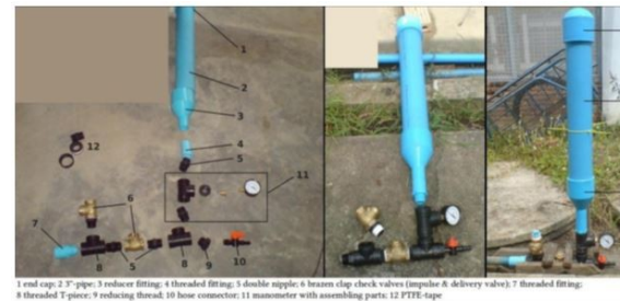
Figure 2. Layout of the described low-cost hydraulic ram to be tested at a test stand and installed remote mountainous areas ( in parts and assembled)
