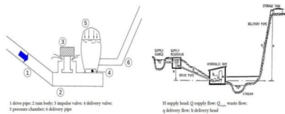
Figure 1. Typical Construction of a hydram (left, according to Abate and Botrel 2002) and its set-up in the field (right, according to tacke 1988)
