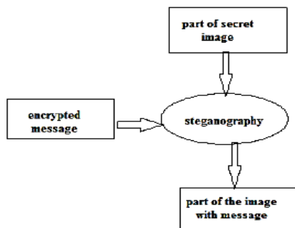
Figure 3: Embedding Phase
