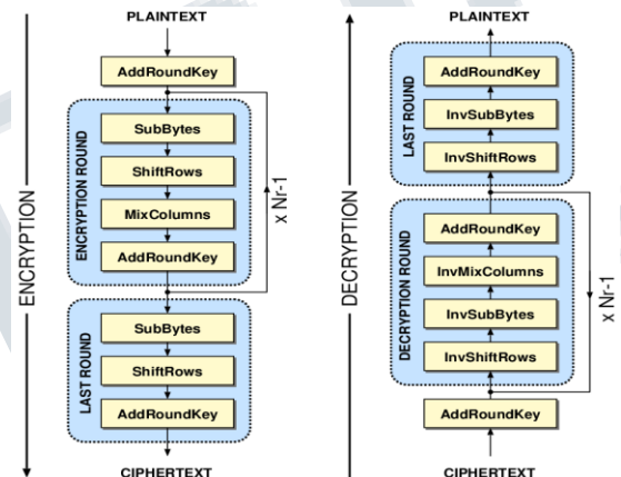
Figure 1 AES Algorithm
