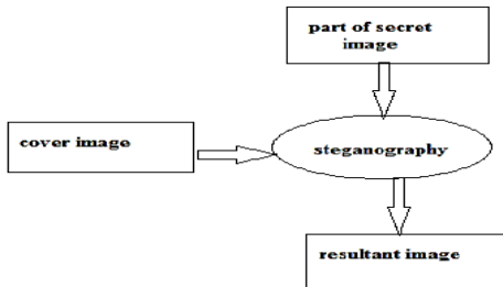
Figure 5 Hiding Phase
