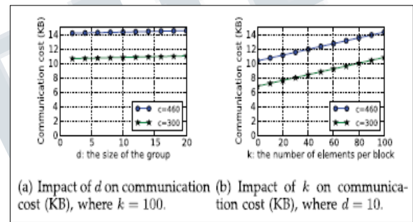
Fig.12. Performance of communication value.
