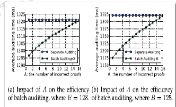
Fig.14. Potency of batch auditing with incorrect proofs.
