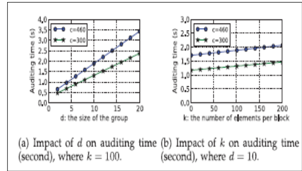
Fig.11. Performance of auditing time.
