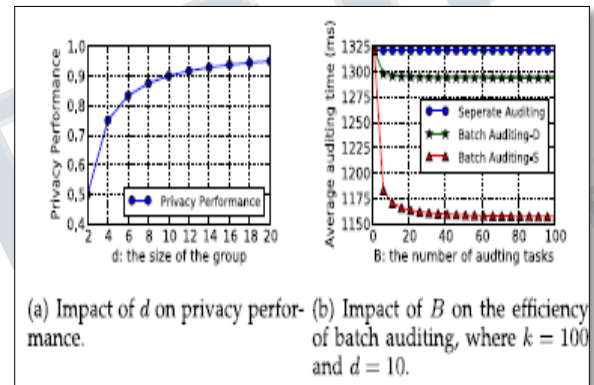
Fig.13. Performance of privacy and batch auditing.
