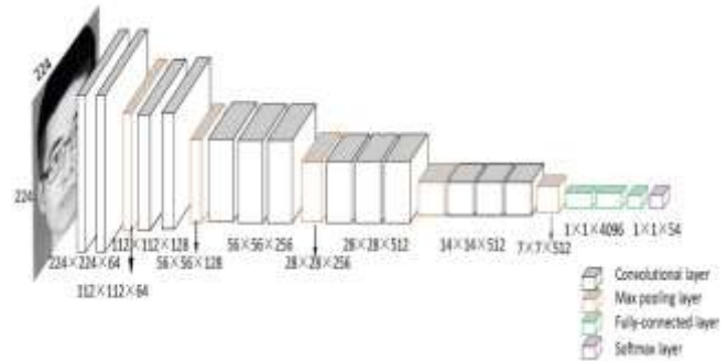
Figure 2. Architecture of the VGG-16 model
