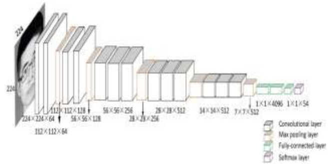
Figure 2. Architecture of the VGG-16 model
