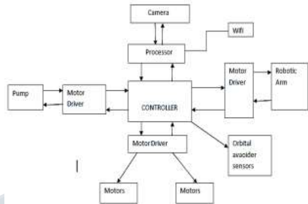
Fig-1: Block diagram for automated ground harvesting machine
