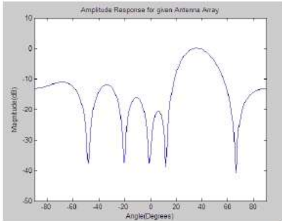
Fig.4 Angle of Arrival Vs Amplitude response: Beam steered at 35° (Signal of interest) and interferer null at -20° and 0° using KLMS algorithm
