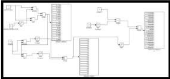
Figure 1. Simulink model
