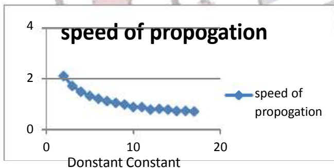
Figure 4 Graphical results (dielectric constant vs. speed of propagation within solid surface)
