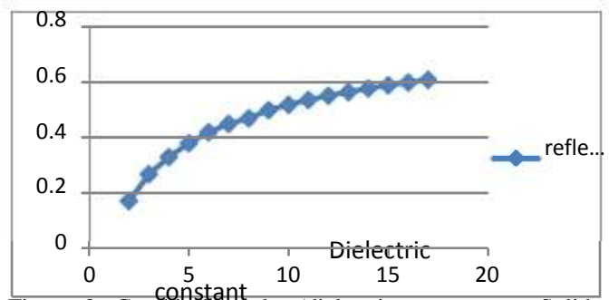
Figure 3. Graphical results (dielectric constant vs. Solid surface reflection coefficient)
