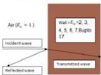
Figure 2, Propagation of EM wave in various mediums
