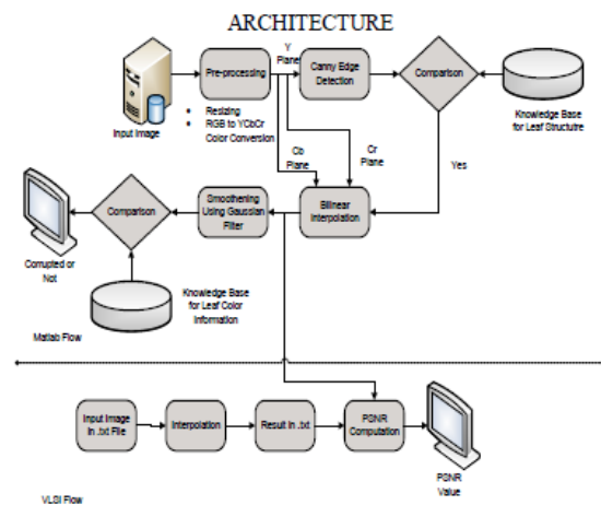
Figure 1: Block Diagram of VLSI Implementation for Color Interpolation
