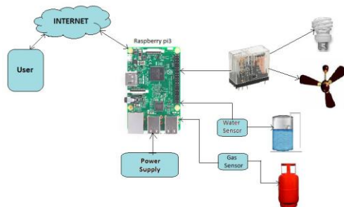
Fig. 4.1 Block diagram of Home Automation Using Raspberry Pi module
