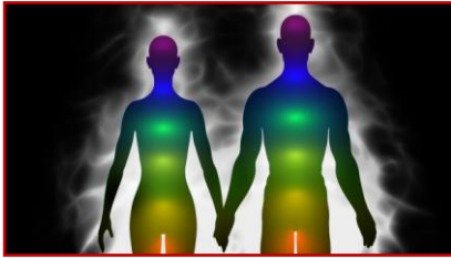
Figure 4: Y-Y Spectrum of Aura
