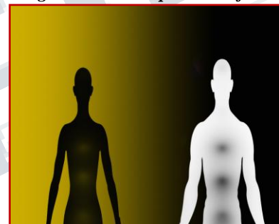
Figure 11: Y-B Spectrum of Aura
