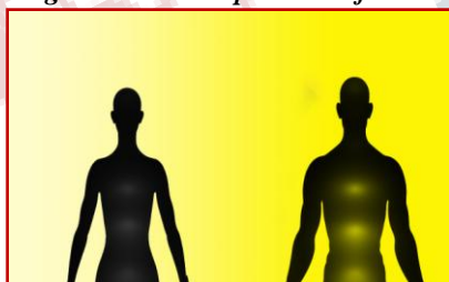
Figure 16: W-Y Spectrum of Aura
