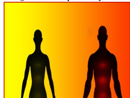
Figure 12: Y-R Spectrum of Aura
