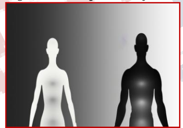
Figure 7: B-W Spectrum of Aura
