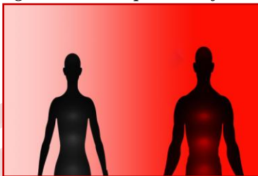
Figure 15: W-R Spectrum of Aura
