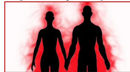
Figure 2: R-R Spectrum of Aura
