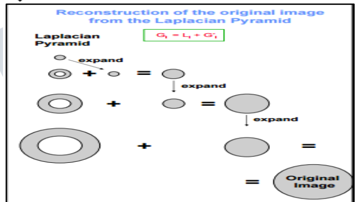
Fig 4: Image construction & Reconstruction using Laplacian Pyramid
