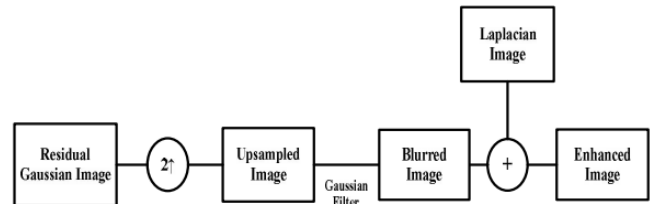
Fig 13: Reconstruction of Laplacian pyramid
