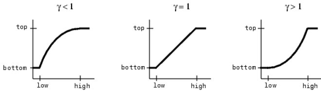
Fig 2: Gamma correction
