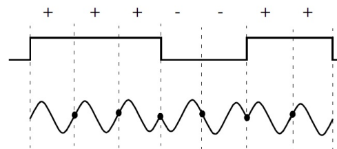
Figure 3. Binary phase code of length 7.
