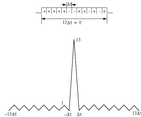
Figure 4. Barker code of length 13 and its corresponding autocorrelation function
