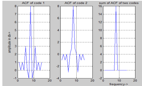
Figure 5. Result for complementary sequence of length 8.
