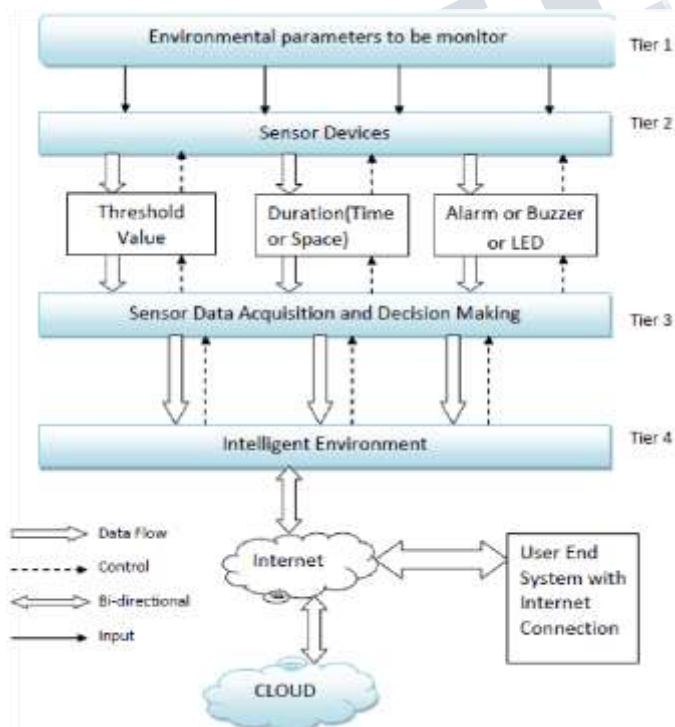
Fig.2: Proposed model
