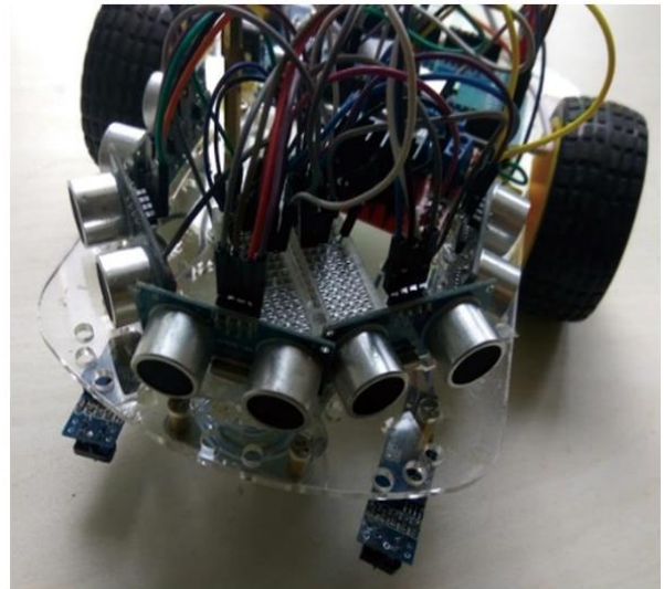
Figure 3. Ultrasonic sensors and infrared sensors
