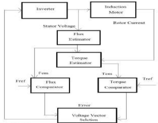
Fig.1. Block Diagram of DTC Method
