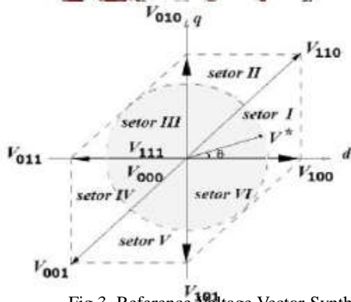
Fig.3. Reference Voltage Vector Synthesis
