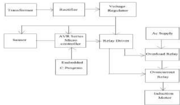
Fig.5. Block Diagram of Motor Protection System
