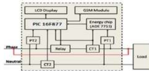
Fig 3.Phase bypassing energy meter
