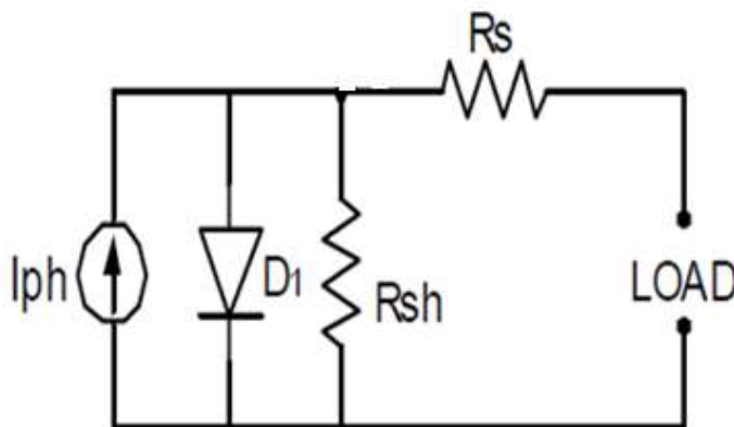
Fig:PV Cell Circuit Model
