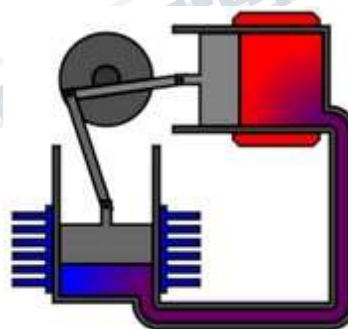
Figure 2: Gas at hot end (red cylinder) expanding isothermally by absorbing heat from the source
