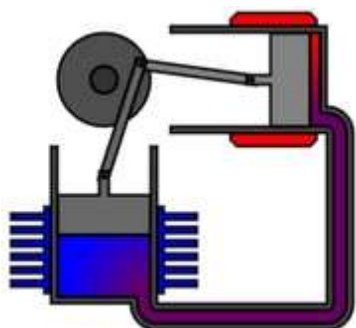
Fig 4: Isothermal compression of the gas from cold end to hot end
