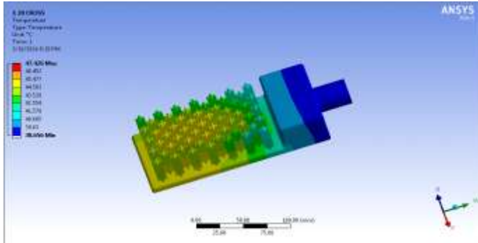
Fig. no.3.2.2 As shown above, after successful run of simulation, found that the maximum temperature reach by base plate by using cross 20mm plus sign fins is near about 47°C, and also by using designing software we know the exact weight of this cross 20mm plus sign finned base plate which is nothing but .66961.Kgs.
