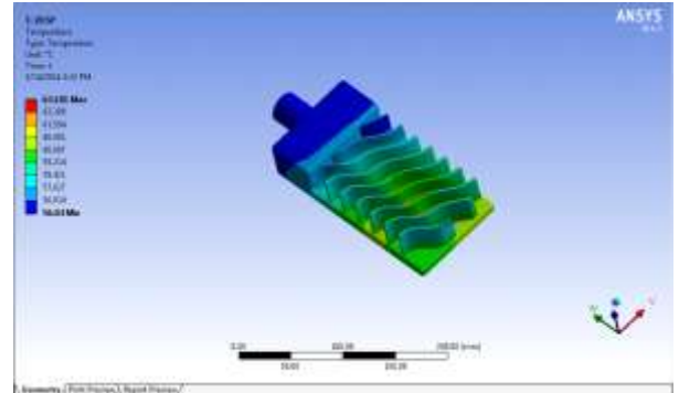
Fig. no.3.2.4 As shown above, after successful run of simulation, found that the maximum temperature reach by base plate by using pline fins is near about 64°C, and also by using designing software we know the exact weight of this spline finned base plate which is nothing but .6065 Kgs.
