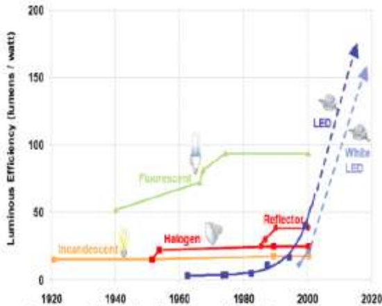
Figure 1. Luminous efficiency timeline for general illumination sources
