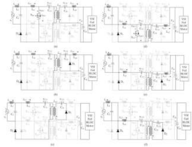
Fig 3-Modes of operation of cuk converter fed BLDC motor
