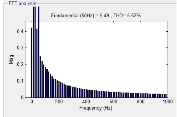
Fig. 11. THD of input current.
