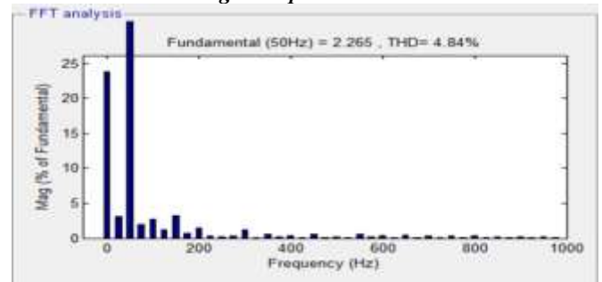
Fig. 7. THD of input current.
