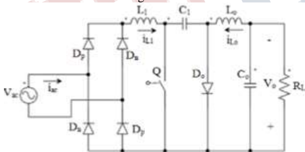
Fig. 1: conventional cuk converter
