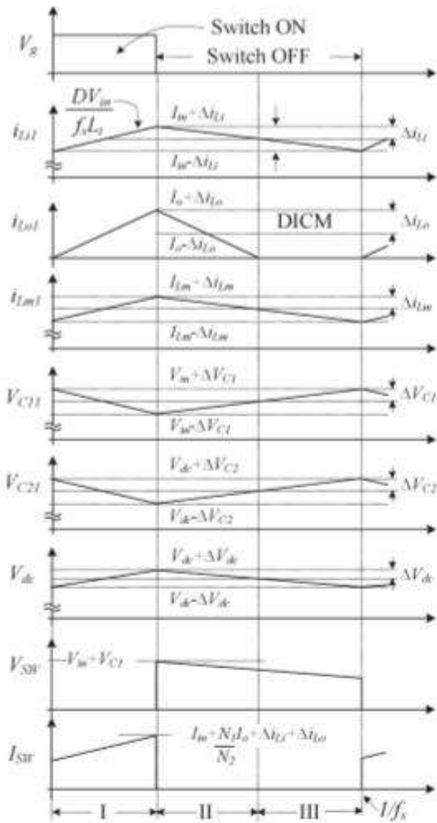
Fig. 4: Waveforms in one switching cycle.
