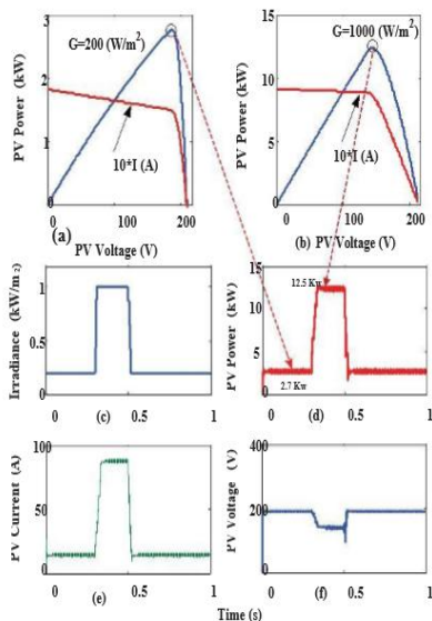
Fig. 5. Simulation results: MPPT Tracking performance of HGICB Converter (a) PV Characteristic at G=200 \text{ W/m}^2 (b) PV Characteristic at G=1000 \text{ W/m}^2 (c) insolation variations (d) PV Maximum Power (e) PV Current (f) PV Voltage
