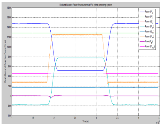
Fig.7. Real and reactive power flow waveforms of PV hybrid generating station
