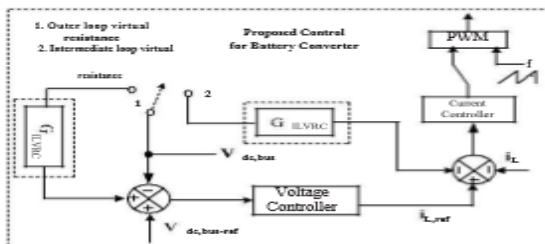
Fig.3.a new modified-ACMC control strategy for battery converter
