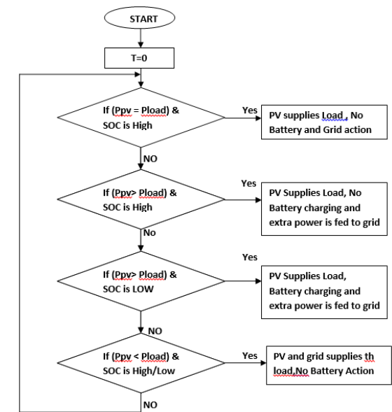
Fig.4.flow chart of power flow in hybrid system
