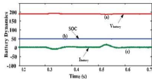
Fig.10. Battery performance using proposed control approach to bi directional battery converter .(a) battery voltage (b) state of charge(SOC) (c) Battery converter
