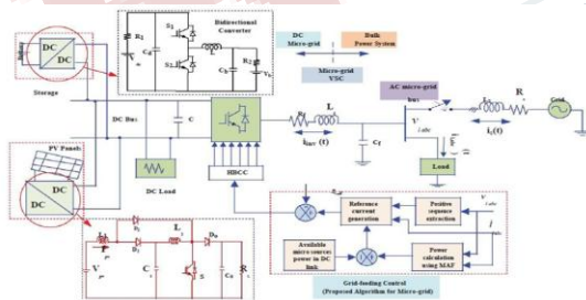
Fig:1 Block Diagram of Hybrid Energy conversion system under consideration
