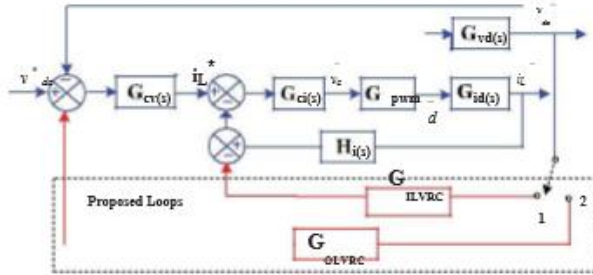
Fig.2.Inner and outer loops of battery converter with MACMC
