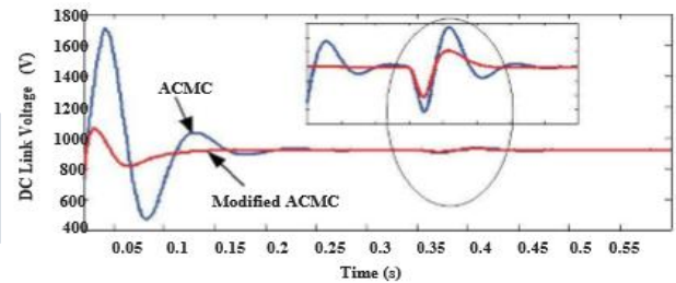
Fig.9. Dc Link Voltage Dynamics Using ACMC And MACMC Control Algorithms
