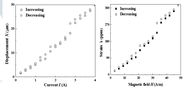
Figure 8. (a) Displacement and (b) strain of a Terfenol-D actuator by varying step input to coil 1 and coil 2.
