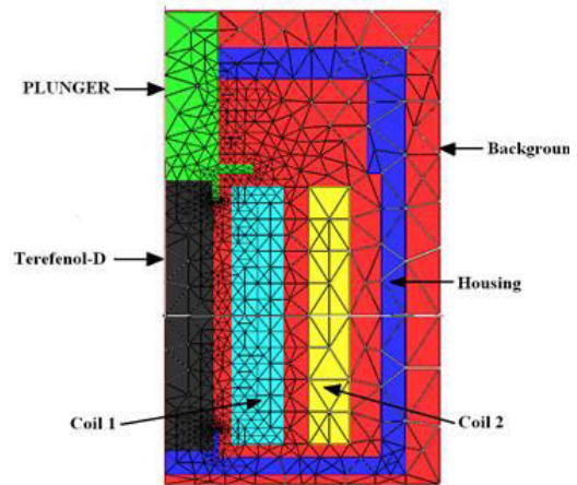
Figure 3. Discretization of the actuator assembly with coaxial coils using triangular finite elements in a Maxwell 2D solver.
