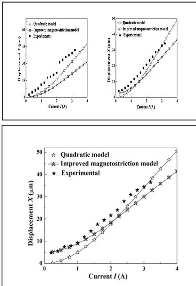
Figure 14. Comparison of theoretical and experimental displacement of a Terfenol-D actuator for different preloads, (a) 0 N (b) 500 N and (c) 1000 N.
