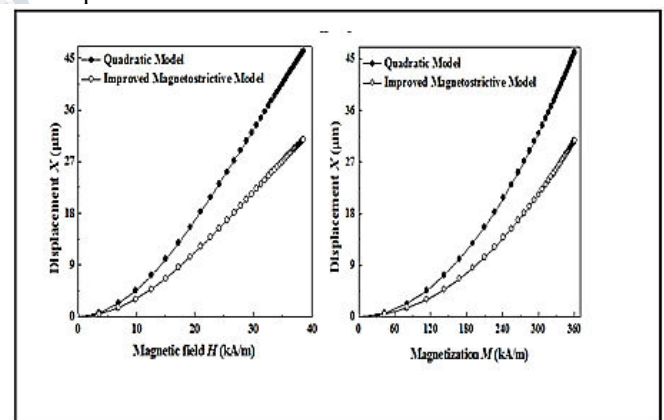
Figure 13. Comparison of theoretical displacement of a Terfenol-D rod as a function of magnetic field (a) and magnetization (b) for a step input of 4 A.
