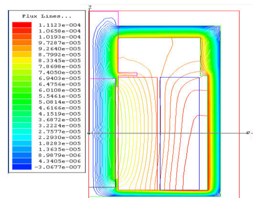
Figure 6. Comparison of flux distribution in an actuator assembly with mild steel housing with Terfenol-D.
