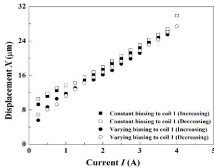
Figure 9. Displacement of a Terfenol-D actuator under biasing conditions.
