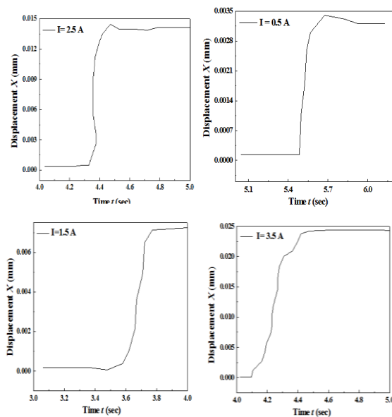
Figure 7. Response of Terfenol-D actuator under zero pre-stress for step input of (a) 0.5 A (b) 1.5 A (c) 2.5 A and (d) 3.5 A to coaxial coils.
