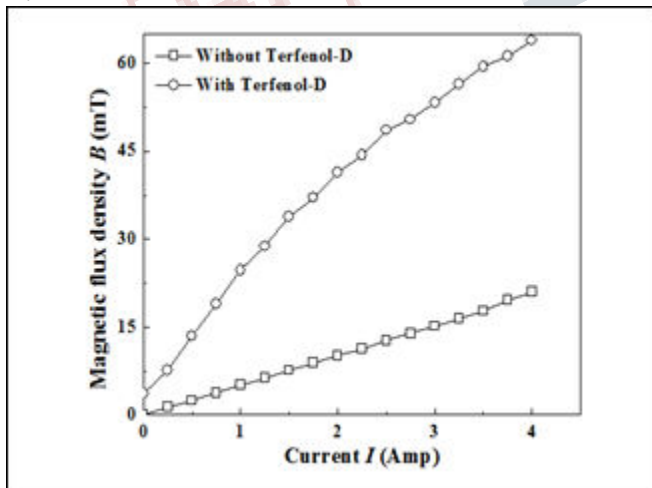
Figure 4. Comparison of magnetic flux density in a coaxial coils with and without Terfenol-D.
