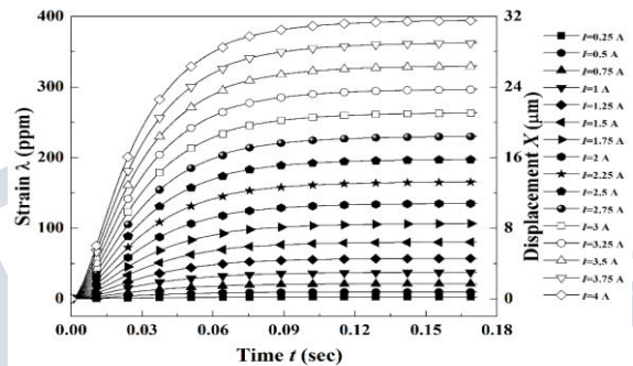
Figure 10. Response characteristics between Magnetic field and magnetization of an actuator as a function of time.
