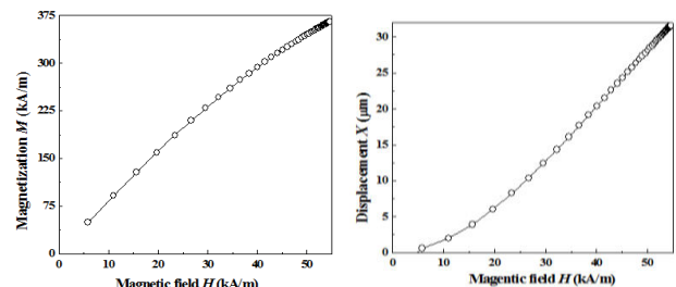
Figure 11. Magnetization curves (a) M vs. H (b) X vs. H of a Terfenol-D actuator.
