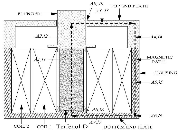
Figure 1. Structure and magnetic circuit of a Terfenol-D actuator.
