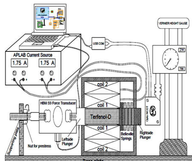
Figure 2(a) . Schematic setup of a Terfenol-D actuator.
