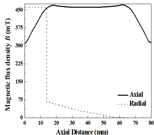
Figure 5. Axial and radial magnetic flux density distribution in an actuator assembly with Terfenol-D.
