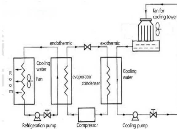
Figure 1: The composition of central air conditioning system
