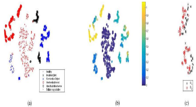
Fig. 6. t-SNE representation of the activity vectors of the output units in the F1rst recurrent layer at the last time step of the sequences in the test data set [h1(2000)]. (a) Labeled by true category. (b) Labeled by fault severity.
