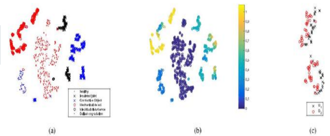
Fig. 7. t-SNE representation of the activity vectors of the output units in the second recurrent layer at the last time step of the sequences in the test data set [h2(2000)]. (a) Labeled by true category. (b) Labeled by fault severity. (c) Ballast degradation sequences labelled per spatial dependence.
