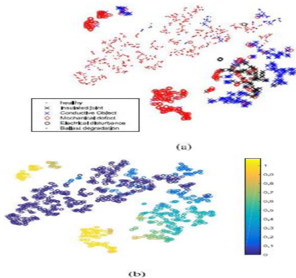
Fig. 6. t-SNE representation of the activity vectors of the output units in the F1rst recurrent layer at the last time step of the sequences in the test data set [h1(2000)]. (a) Labeled by true category. (b) Labeled by fault severity.
