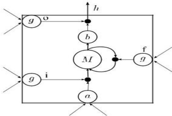
Fig. 2. Architecture of the LSTM memory cell. Black dots: multiplication of the outputs of the gate units g by the outputs of the regular units.
