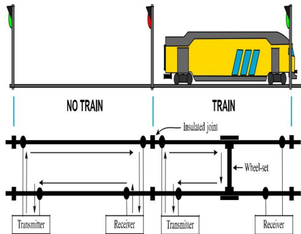
Fig. 1. Current flow in a track circuit. Each track circuit detects the absence of trains in a section of a railway track. Subsequent sections are separated from each other by insulated joints.
