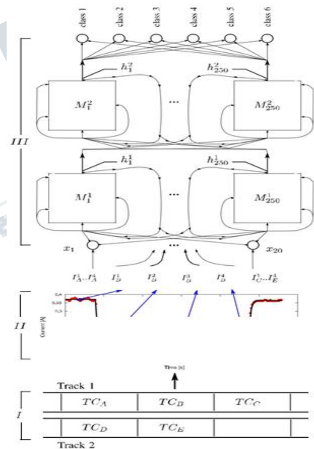
Fig. 3. Fault diagnosis process overview. For each train-passing event T, the current time sequence of the Five track circuits (I) is sampled (II). These samples are the input to the neural network (III), which uses them to update the likelihood P(Y = c)(T) of the six different fault classes.
