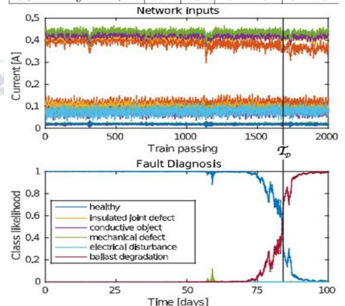
Fig. 4. Network inputs and output for one realization of a ballast degradation fault sequence. The detection time T_D marks the detection threshold. Before this point, the correct classification is healthy, and after this point, the correct classification is ballast degradation.
