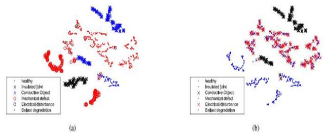
Fig. 8. t-SNE representation of the state of the memory units in the second recurrent layer at the last time step of the sequences in the test data set [M2 (2000)]. (a) Labeled by true category. (b) Separating conductive objects from electrical disturbances
