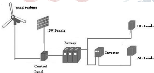
Fig.2.Hybrid energy system
