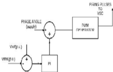
Fig.3. SPWM Control
