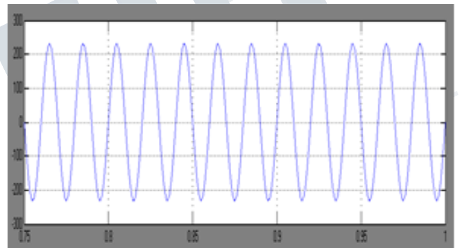
Fig.8. Output Voltage with D-STATCOM
