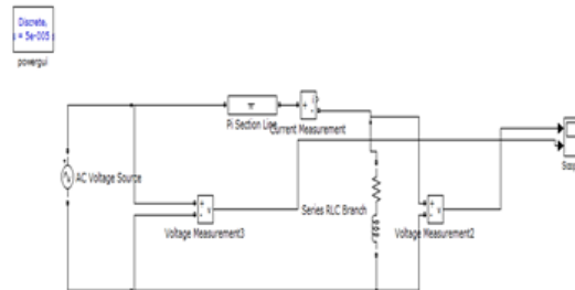
Fig. 4. Simulation without DSTATCOM
