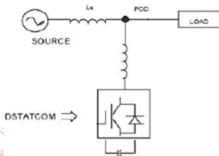
Fig.1. Block diagram DSTATCOM circuit.
