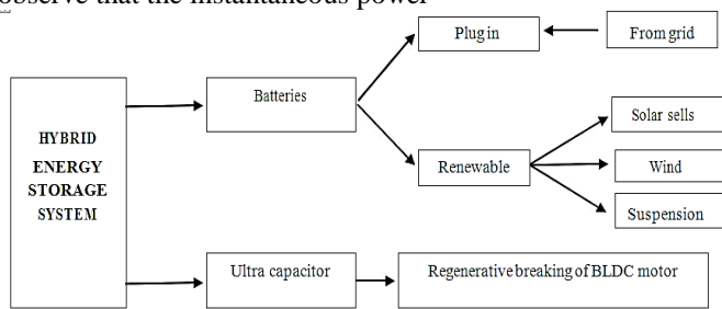
Fig.2:- Energy storage system and charging structure
