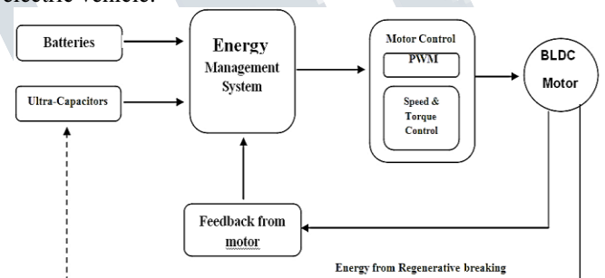
Fig.3:- Energy Management System
