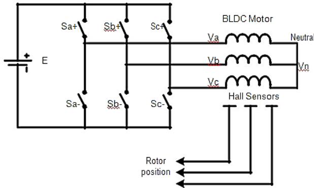
Fig. 1:- Structure of BLDC motor connected to inverter
