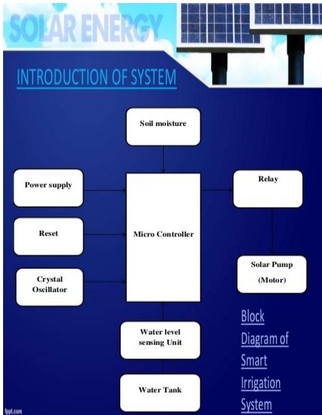
Fig.1. block diagram of smart irrigation system Implementation:
