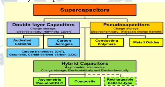
Fig3. Types of supercapacitors
