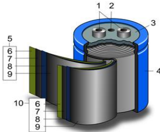
Fig4. Schematic construction of a wound supercapacitor
