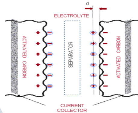
Fig2. schematic diagram of supercapacitor
