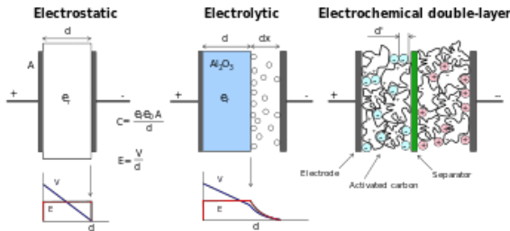
Fig1. supercapacitor diagram
