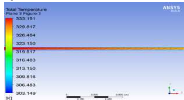
Fig. 3. For 9 LPM mass flow rate and 4.4 twist ratio
