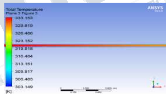
Fig. 2. For 9 LPM mass flow rate
