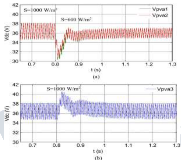
Fig. 6. DC-link voltages of phase a with distributed MPPT ( T = 25 \text{ }^\circ\text{C} ). (a) DC-link voltage of modules 1 and 2. (b) DC-link voltage of module 3.
