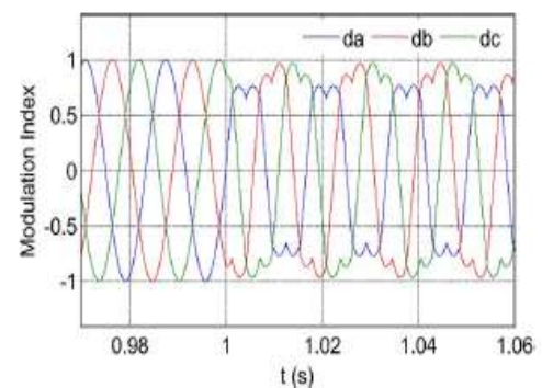
Fig. 5. Modulation indices before and after modulation compensation
