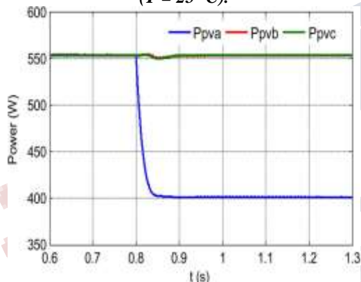
Fig. 12. Power injected to the grid with modulation compensation.
