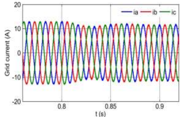
Fig. 14. Three-phase grid current waveforms with modulation compensation
