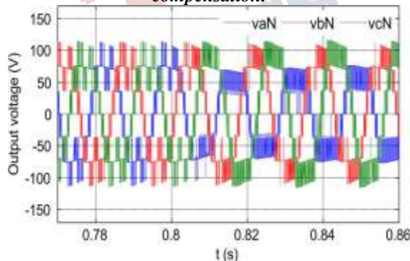
Fig. 13. Three-phase inverter output voltage waveforms with modulation compensation.
