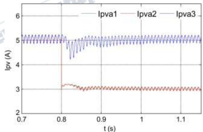
Fig. 7. PV currents of phase a with distributed MPPT ( T = 25 \text{ }^\circ\text{C} ).
