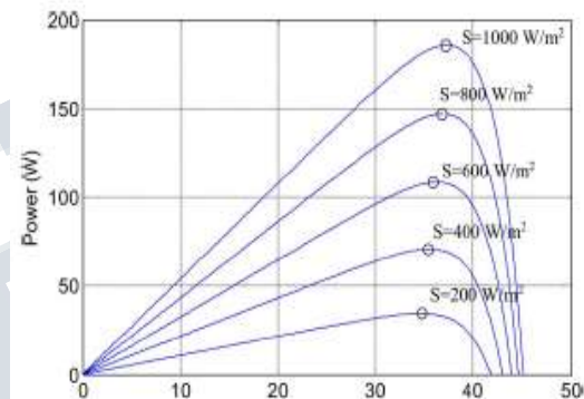
Fig. 3. P-V characteristic under the different irradiance.
