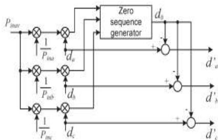
Fig. 4. Modulation compensation scheme
