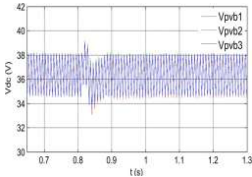
Fig. 10. DC-link voltages of phase b with distributed MPPT ( T = 25\text{ }^{\circ}\text{C} ).
