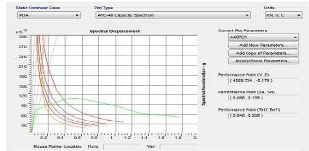
Fig. 8- Capacity spectrum curve for regular building
