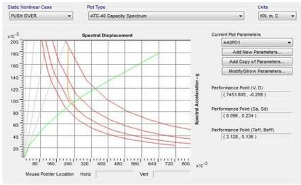
Fig. 8- Capacity spectrum curve for setback 4 building
