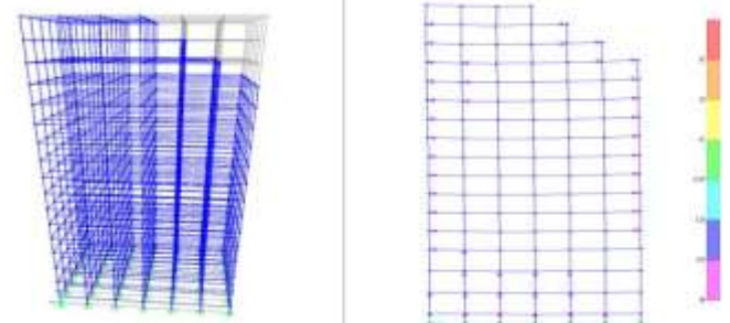
Fig. 13- Hinge formation for setback 4 building
