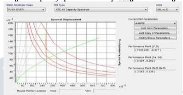
Fig. 8- Capacity spectrum curve for setback 1 building
