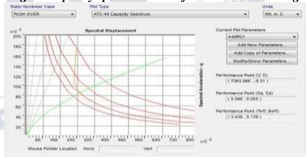
Fig. 8- Capacity spectrum curve for setback 2 building
