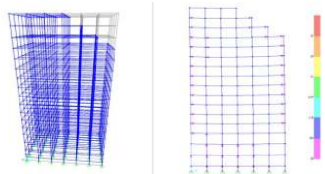
Fig. 12- Hinge formation for setback 3 building
