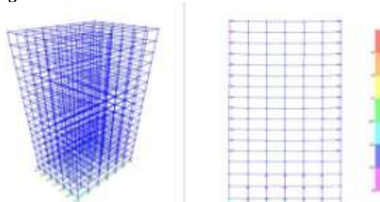
Fig. 9- Hinge formation for regular building
