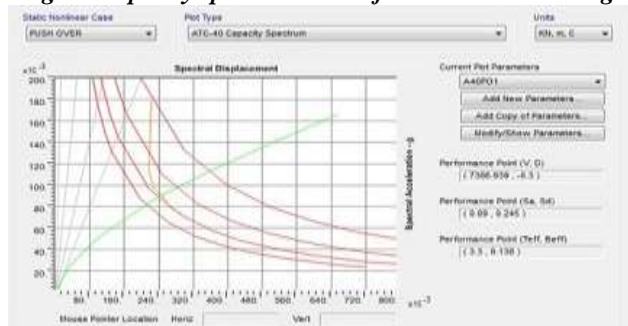
Fig. 8- Capacity spectrum curve for setback 3 building
