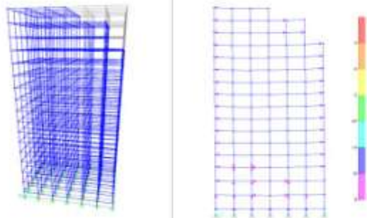
Fig. 11- Hinge formation for setback 2 building
