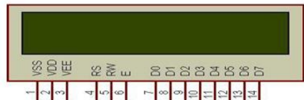
Figure6. Character LCD type Pin diagram.
