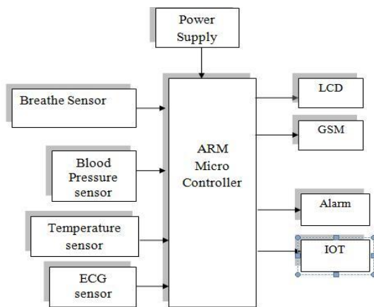
Figure1.The general block diagram of the components.
