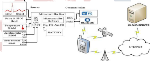
Figure7. Monitoring device's block diagram and network structure
