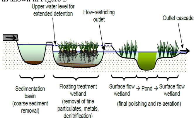
Figure 2- Conceptual Design of Storm Water Treatment (Source: Headley and Tanner (2008))
