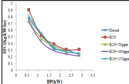
Figure 4. Variation of Specific fuel consumption with B.P
