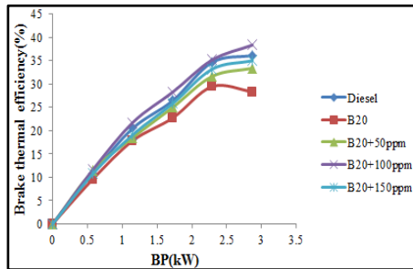
Figure 3. Variation of Brake thermal efficiency with B.P
