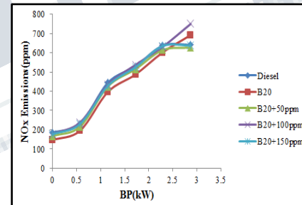
Figure 7. Variation of NO x Emissions with B.P
