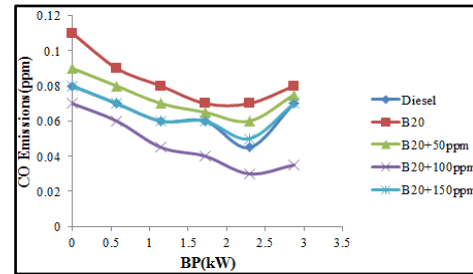
Figure 6. Variation of CO Emissions with B.P
