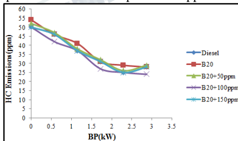
Figure 5. Variation of HC Emissions with B.P
