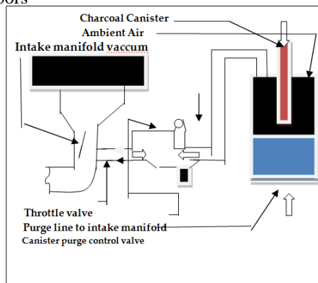
Figure: 2(a) Evaporative Emission Control System
