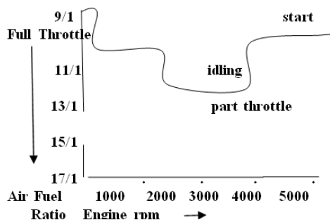
Fig: 3(a) Graph/- Air Fuel Ratio/Engine rpm
