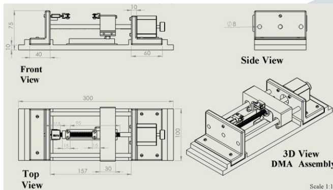
Figure.1 Computer Aided Drafted view of DMA system.
