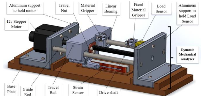
Figure.2 SolidWork Assembly of CAD Model for designed DMA system.
