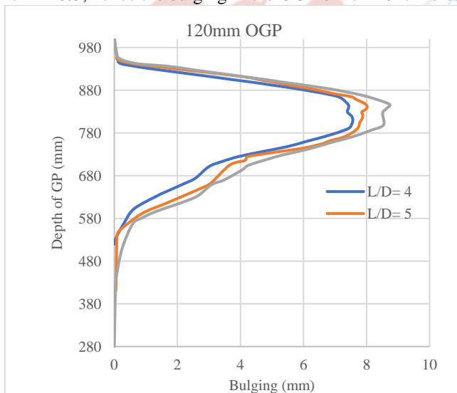
Fig.6 Variation of the bulging with depth for OGP of 100mm diameter
