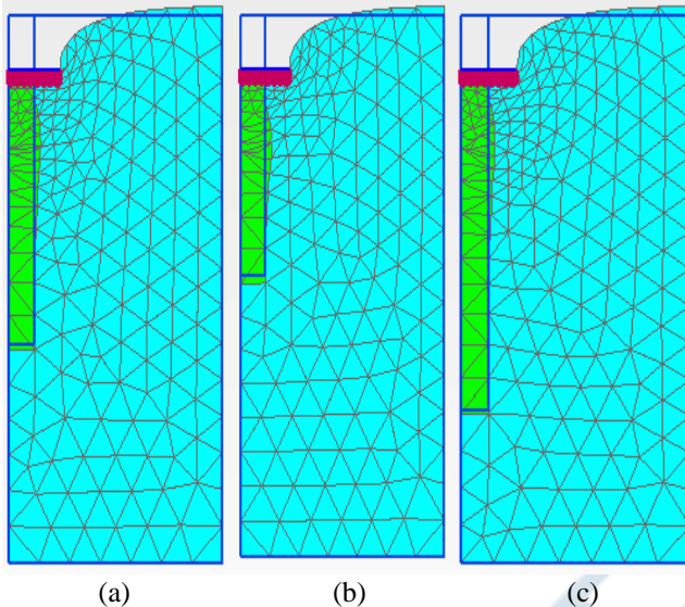
Fig.5 (a,b,c) Represents Bulging in OGP of 120 mm diameter, of L/D = 4,5 and 6
