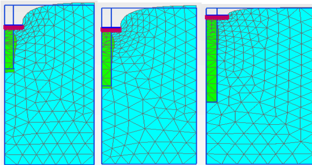
Fig. 1 (a, b, c) Represents Bulging of OGP of 80mm diameter, for L/D 4,5, and 6 respectively
