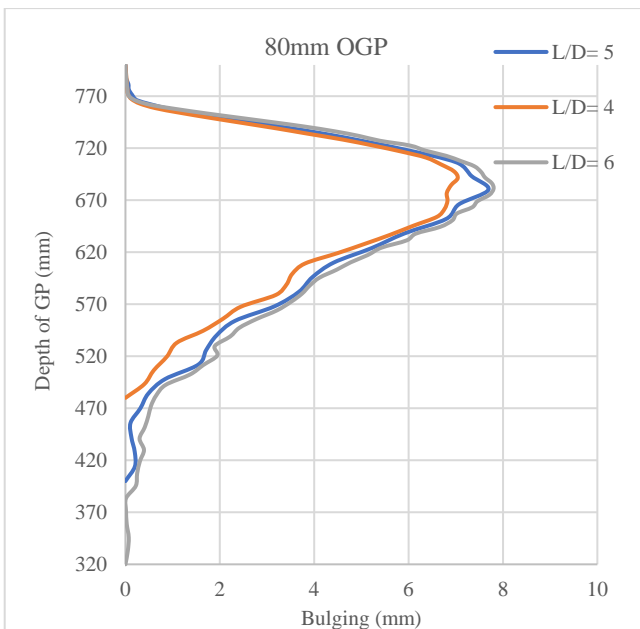
Fig.2 Variation of Bulging with Depth of the OGP for 80mm diameter OGP
