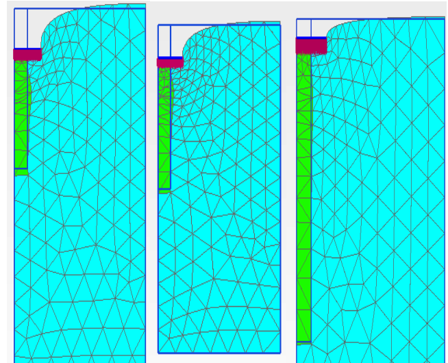
Fig.3 (a, b, c) represents Bulging of OGP of 100mm diameter for L/D 4,5 and 6
