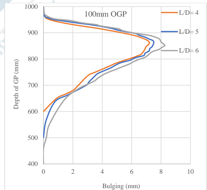
Fig.4 Variation of the bulging with depth for OGP of 100mm diameter
