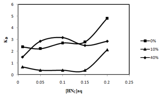
Fig. 2: Chemical extraction of Methylsuccinic acid by sesame oil with TBP. Variation of distribution coefficient (KD) with initial aqueous phase acid concentration.
