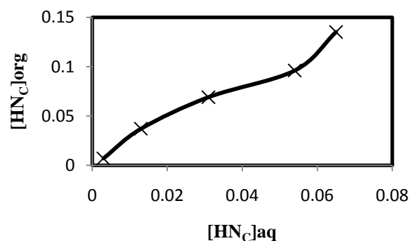
Fig. 1: Physical equilibria for extraction of Methylsuccinic acid using sesame oil at 298 K.
