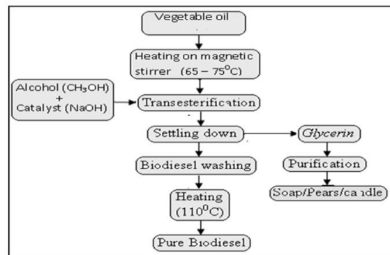
Fig.1 Flow chart of Biodiesel production.
