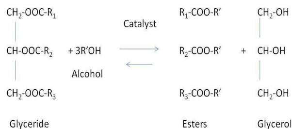
Fig. 2 Transesterification of triglycerides with alcohol in presence of catalyst, where R is the alkyl group.
