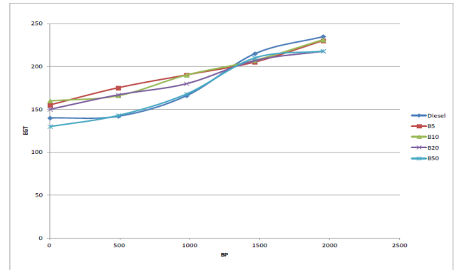
Fig. 6 Exhaust gas temperature Vs Break power.
