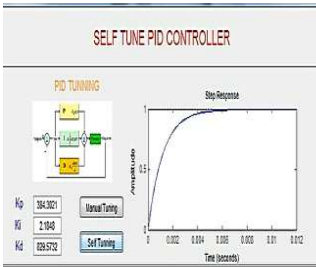
Figure 1.2 Step response of the proposed system at auto tuned PID gain parameters
