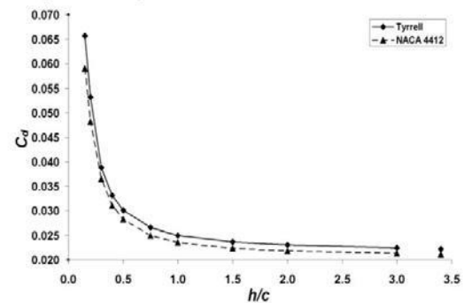
Fig. – 3 C_d vs h/c , data of Jonathan W. Vogt et al. [8]
