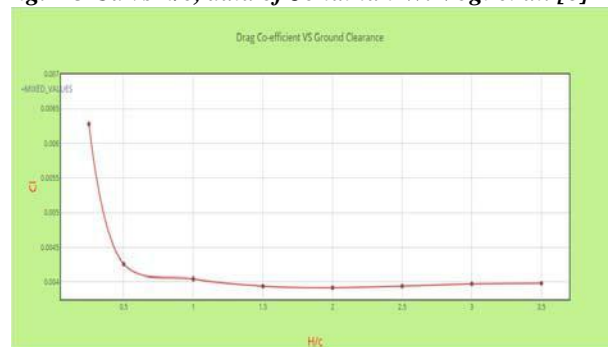
Fig. – 4 C_d vs h/c of calculated data for rear wing of car.
