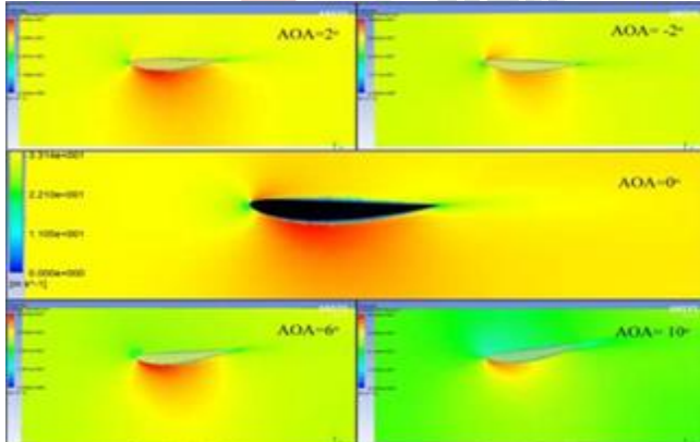
Fig.- 10 Velocity Variation of NACA 4412 at 180 KMPH
