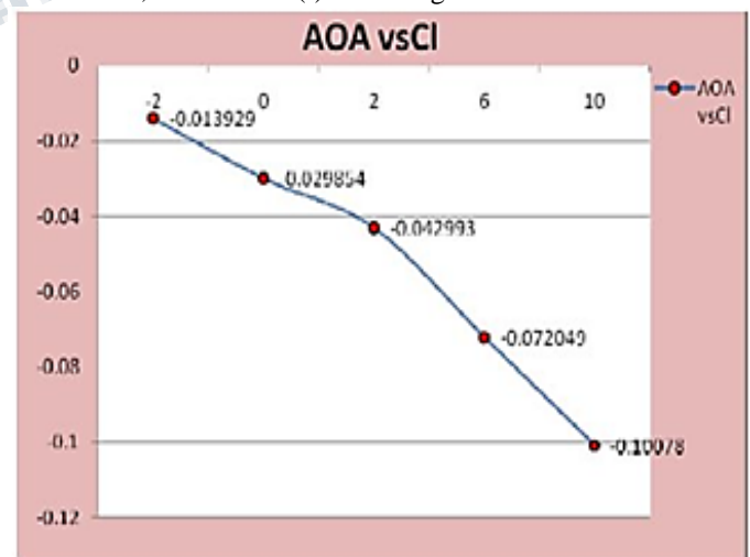
Fig. – 7 AOA vs Cl for 180 KMPH
