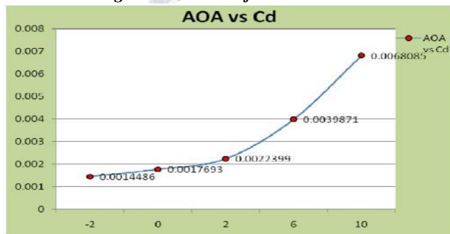
Fig. – 6 AOA vs Cd for 120 KMPH
