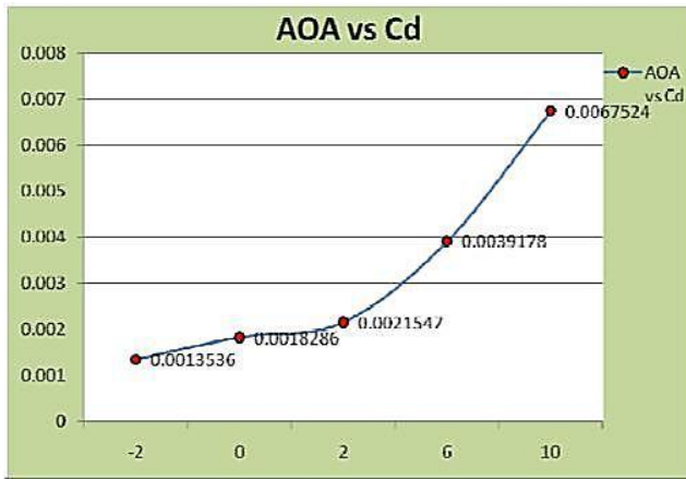
Fig. - 8 AOA vs Cd for 180 KMPH
