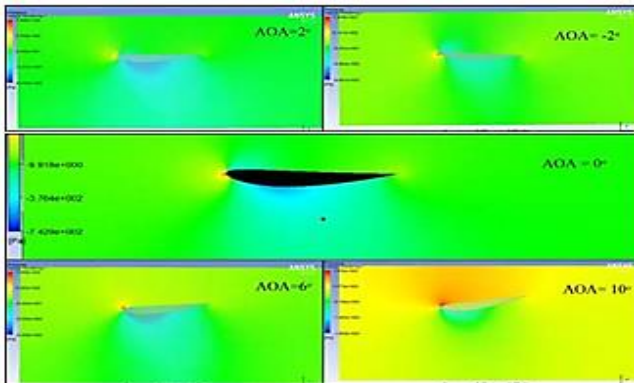
Fig.- 9 Pressure distribution for NACA 4412 at 120 KMPH
