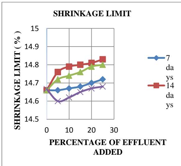
Fig.3. Variation in Shrinkage limit of red soil mixed with soap effluent
