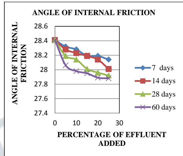
Fig. 7. Variation in Angle of Internal Friction of red soil mixed with soap effluent
