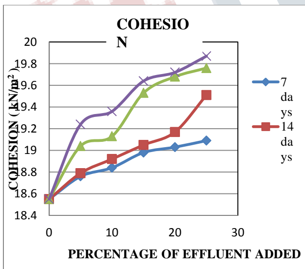
Fig. 6. Variation in Cohesion of red soil mixed with soap effluent
