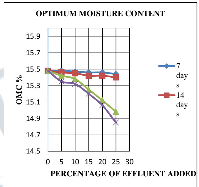
Fig. 5. Variation in OMC of red soil mixed with soap effluent
