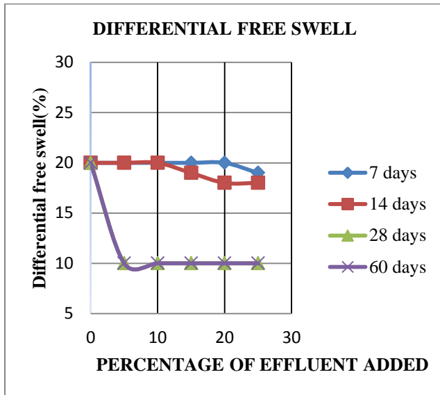
Fig. 6. Variation in DFSI of red soil mixed with soap effluent
