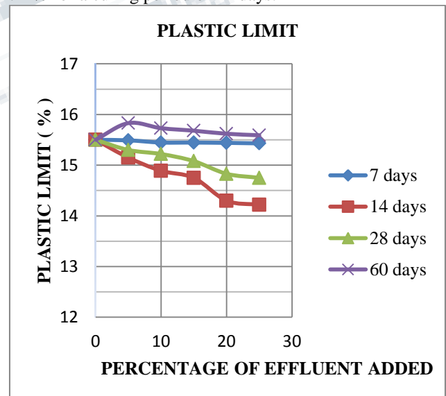
Fig. 2. Variation in Plastic limit of red soil mixed with soap effluent
