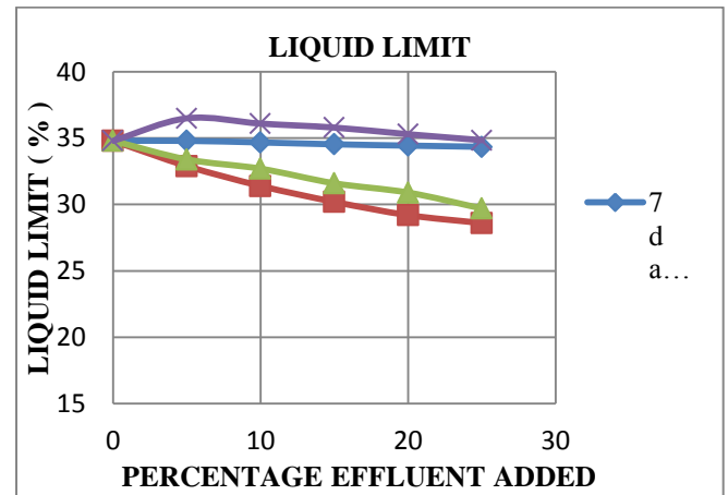
Fig. 1. Variation in liquid limit of red soil mixed with soap effluent
